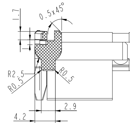
SECTION A-A SCALE 2
