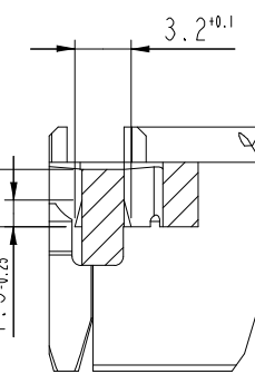
SECTION E-E SCALE 2
