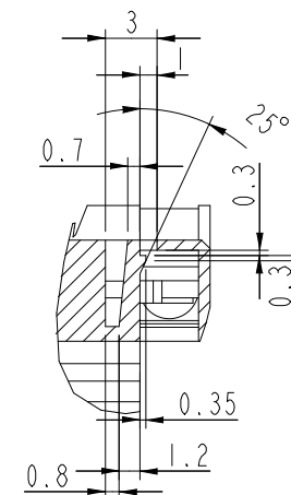
SECTION D-D SCALE 2
