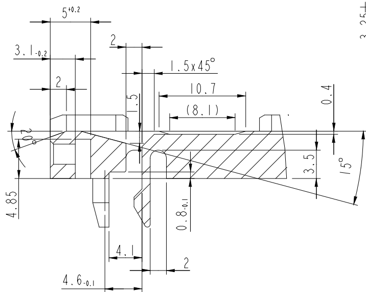
SECTION C-C SCALE 2
