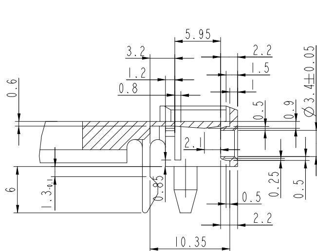
SECTION B-B SCALE 2
