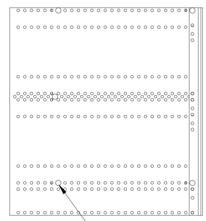
Detail X
