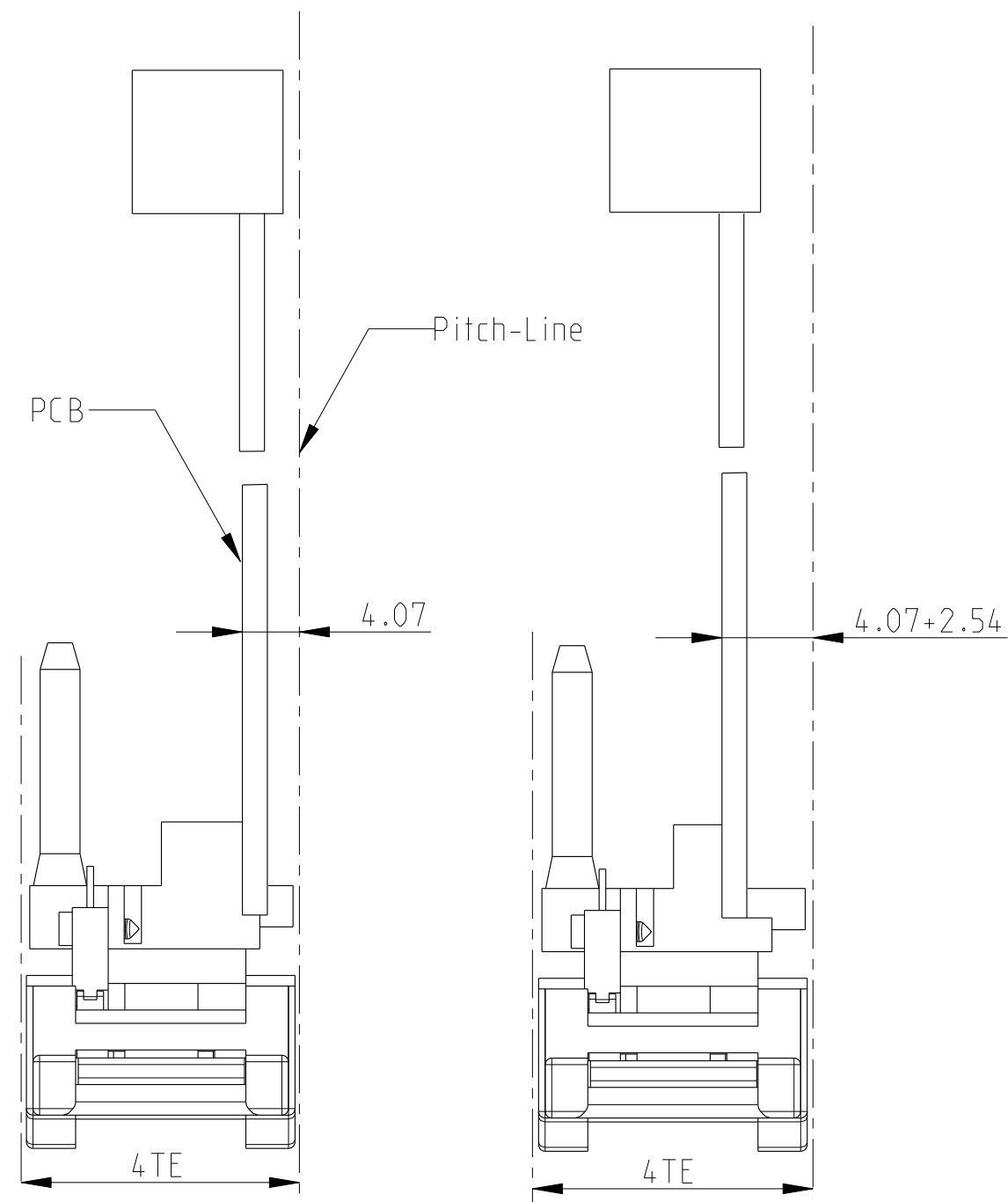
single part no.: 3688782 kit no.: 3688784 Handle Typ VII top without offset
